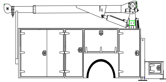
STREET SIDE VIEW
