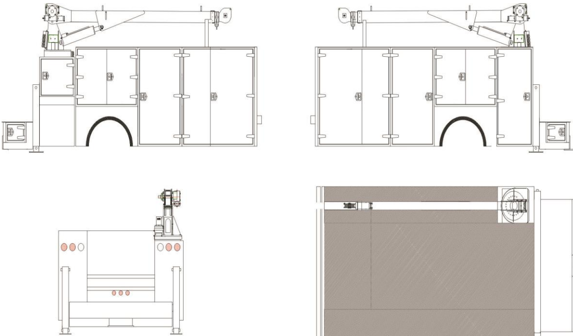
CRANE CAN BE MOUNTED EITHER STREET OR CURB SIDE
