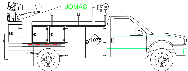
Required Cab to center of axle dimension is 84"
