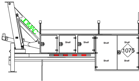
MIDSHIP CABINET PROFILE
